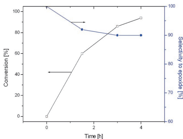
Figure 2. Conversion of 1-methyl-1-cyclohexene and selectivity to epoxide as a function of time at 298 K and 14.5 psi oxygen pressure.
