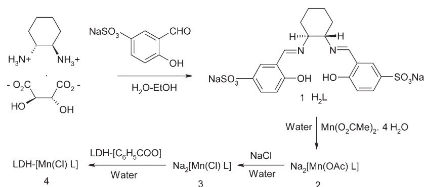
Scheme 1. Preparation of chiral sulphonato-manganese (III) and the LDH-hosted catalyst.
