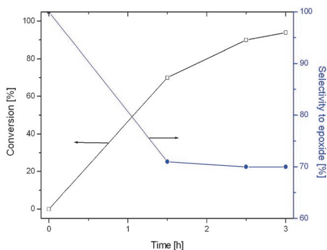
Figure 1. Conversion of 4-methylstyrene and selectivity to epoxide as a function of time at 298 K, 14.5 psi oxygen pressure.
