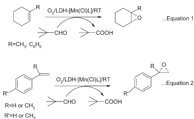
Scheme 2. LDH-hosted Mn-salen-catalysed epoxidation of cyclic alkenes and styrenes in the presence of pivalaldehyde.
