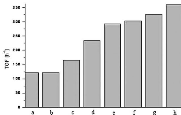
Figure 3. Comparison of TOF (h -1 ) of: (a) cyclohexene, (b) styrene, (c) 1-phenyl-1-cyclohexene, (d) 1-methyl-1-cyclohexene, (e) R -(+)-limonene, (f) (-)- \alpha -pinene, (g) 4-methylstyrene, and (h) \alpha -methylstyrene, over LDH hosted Mn-salen catalyst.
